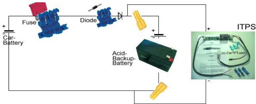
Backup-Battery-Wiring-Diagram
